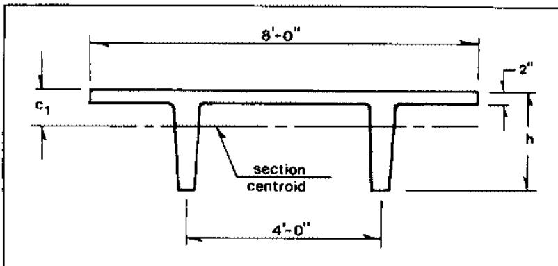
Fig. 6. Double tee beam cross section for Example 2.
