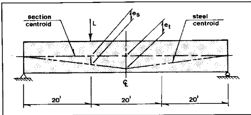
Fig. 4. Beam elevation for Example 1.
