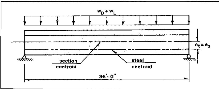
Fig. 5. Beam elevation for Example 2.
